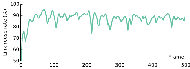
Figure 7: Reuse of Collision Links: In a typical hair simulation, our temporally coherent link update reuses more than 80% of links from previous frames on average.
