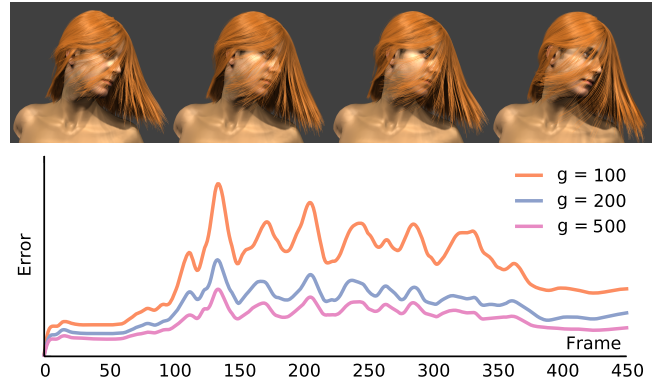
Figure 10: Effects of number of guide hairs: (Top) one resulting frame simulated using 100/200/500 guide hairs and a full simulation. (Bottom) the respective reconstruction error curves of a training sequence, evaluated according to Eq. (8).
