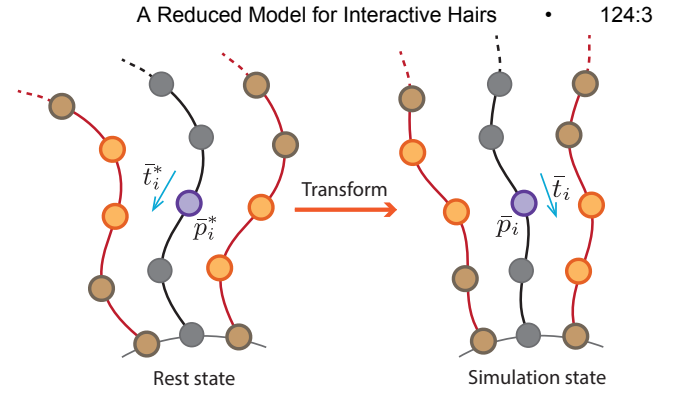
Figure 3: Hair Skinning Model: In our hair skinning model, each normal hair particle (in purple) is interpolated from its guide hair particles (in orange). (Left) We describe the rest state of a hair particle using a tangential vector \bar{t}_i^* and particle position \bar{p}_i^* in the head's local frame of reference. (Right) We use the skinning model Eq. (2) to interpolate normal hair particles also in the head's frame of reference.
