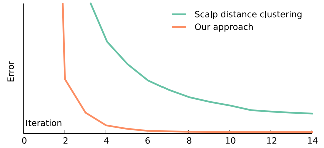
Figure 8: Error convergence curves of iterative hair correction with different particle clustering strategies: The error is defined as the sum of particle distances to the directly solved optimal particle positions. The green curve is generated using a naive clustering based on geodesic distance of strand roots on head scalp. The orange curve shows the result with our hair correction groups, which requires much fewer iterations to converge.
