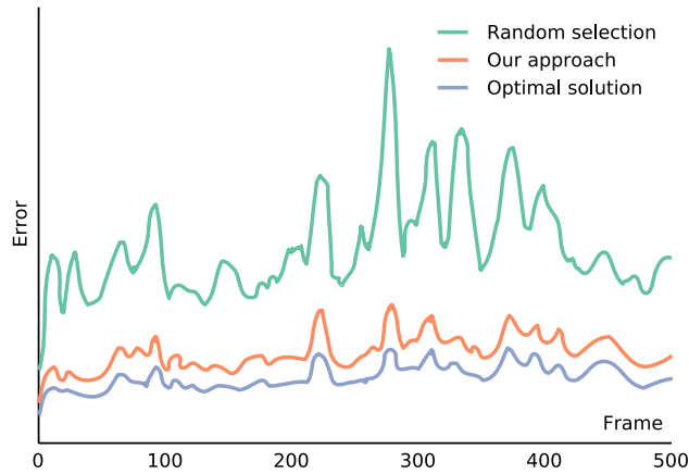
Figure 6: Reconstruction Errors of different guide hair selection strategies: the error metric is defined as Eq. (8). Randomly selected guide hairs (green curve) lead to large error. A brute-force hair selection strategy (blue curve) performs iteratively over every group to find the guide strands that lead to the smallest error, taking about 10 hours. Our heuristic approach (orange curve) is slightly less optimal, but much faster, taking less than 10 minutes.
